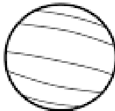
Neptune
