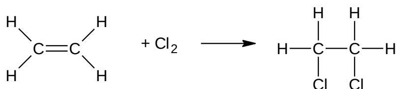
1, 2-dichloroethane
